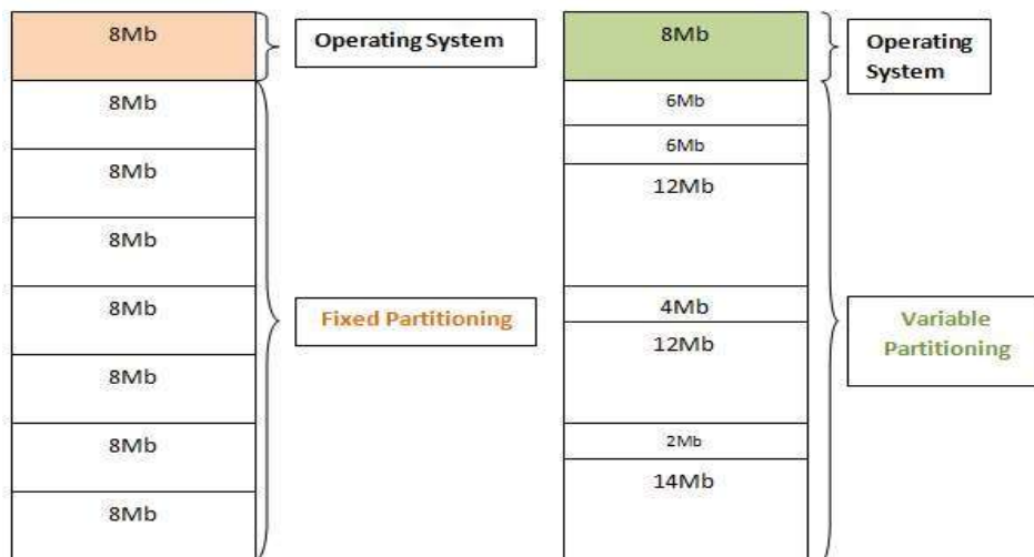
Figure 4: Fixed Partitioning
